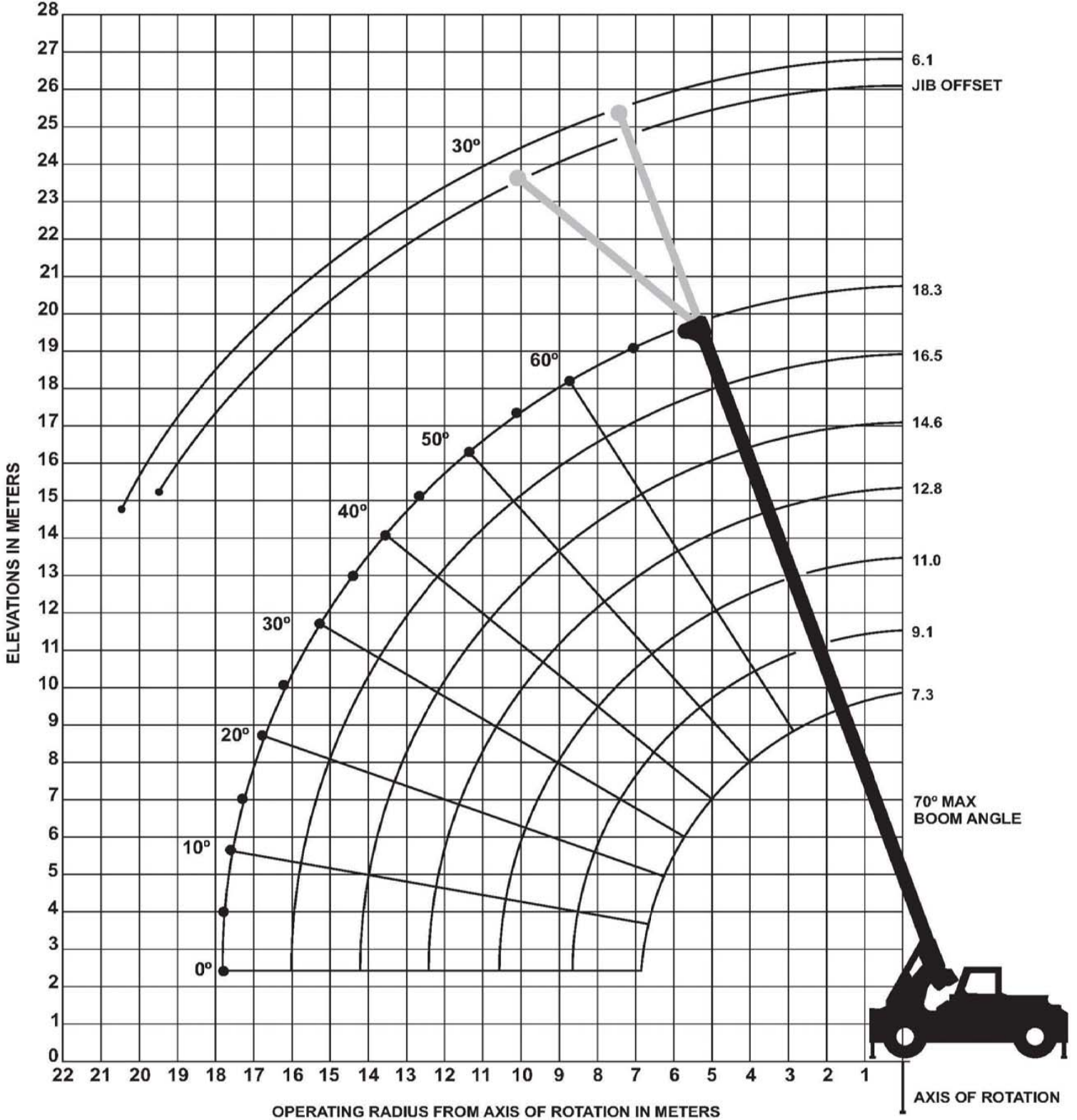
RANGE DIAGRAM (UNLADEN BOOM)
